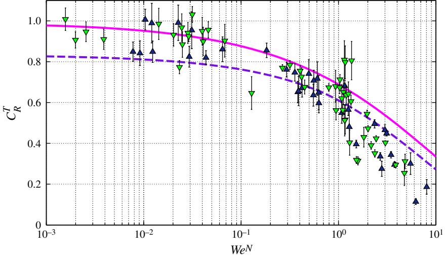
FIGURE 7. (Colour online) The tangential coefficient of restitution C_R^T = v_{out}^T/v_{in}^T as a function of the normal Weber number We^N = \rho R_0 (v_{in}^N)^2 / \sigma , where v^T and v^N are the tangential and normal components of the drop velocity relative to the bath surface. Data for 20 cSt ( \blacktriangledown ) and 50 cSt ( \blacktriangle ) silicone oil are shown, together with the values obtained with the model (4.1) with C = 0.3 for R_0 = 0.1 mm (solid line) and R_0 = 0.4 mm (dashed line). The impact angle with respect to the bath surface ranged from 45^\circ to nearly 90^\circ .
