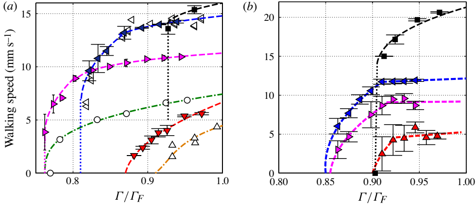
FIGURE 5. (Colour online) The walking speed of silicone oil droplets for (a) \nu = 20 \text{ cSt} , f = 80 \text{ Hz} and (b) \nu = 50 \text{ cSt} , f = 50 \text{ Hz} , bouncing on a vibrating bath of the same oil, as a function of the driving acceleration. The experimentally measured speeds are shown for several droplet radii R_0 . For 20 \text{ cSt} , R_0 = 0.31 \text{ mm} (▼), 0.38 \text{ mm} (►), 0.40 \text{ mm} (◄) and 0.43 \text{ mm} (■); while for 50 \text{ cSt} , R_0 = 0.25 \text{ mm} (▲), 0.34 \text{ mm} (►), 0.39 \text{ mm} (◄) and 0.51 \text{ mm} (■). In panel (a), the walking speeds reported by Protière et al. (2006) are also shown for comparison, for drop radii 0.28 \text{ mm} (Δ), 0.35 \text{ mm} (○) and 0.41 \text{ mm} (◁).
