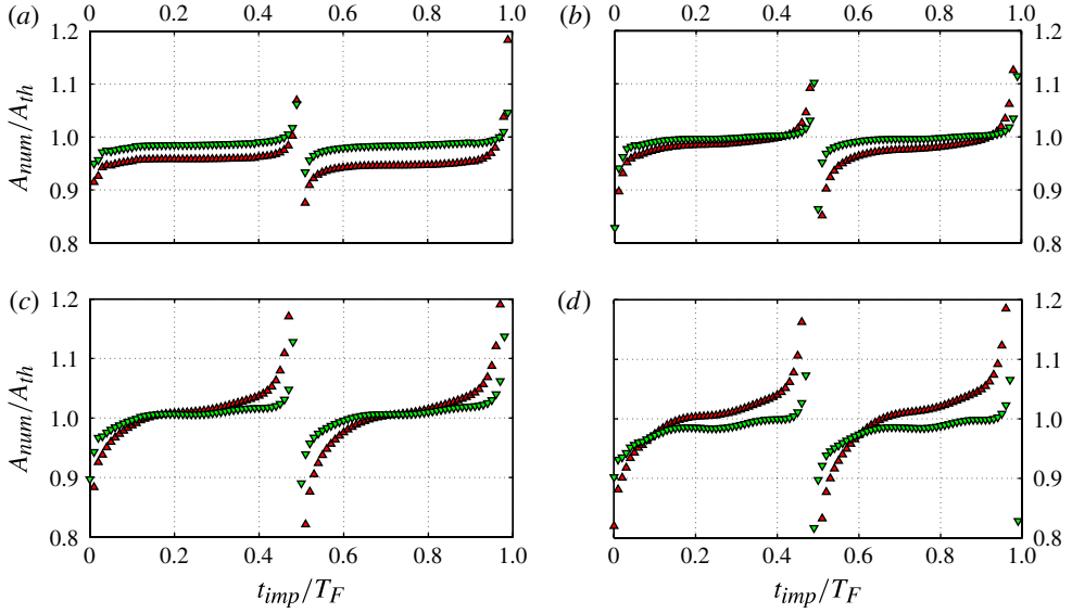
FIGURE 18. (Colour online) Comparison between the full numerical model and the long-term approximation (A 52). The bath surface is forced at time t = t_{\text{imp}} and then evolved freely, and the amplitude of the standing wave A(t) = h(0, t) is recorded, as computed by a full numerical scheme solving (A 27) ( A_{\text{num}} ) and as given by (A 52) ( A_{\text{th}} ). The average ratio A_{\text{num}}/A_{\text{th}} over T_F \leq t \leq 6T_F ( \blacktriangle ) and over T_F \leq t \leq 10T_F ( \blacktriangledown ) is shown as a function of t_{\text{imp}} , for different combinations of oil viscosity and driving frequency: (a) \nu = 10 cSt and f = 100 Hz; (b) \nu = 20 cSt and f = 80 Hz; (c) \nu = 50 cSt and f = 50 Hz; and (d) \nu = 100 cSt and f = 40 Hz. The ratio tends to 1 for large times, except near t_{\text{imp}} \approx (n/2)T_F , when G_1(t_{\text{imp}}) \approx 0 and other wavenumbers contribute to the overall amplitude beside the region near k_F .
