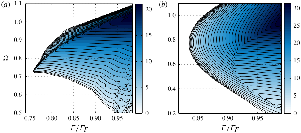
FIGURE 14. (Colour online) The walking speeds ( \text{mm s}^{-1} ) obtained with our model for (a) \nu = 20 cSt at f = 80 Hz and (b) \nu = 50 cSt at f = 50 Hz. The horizontal axis indicates the ratio of the peak driving acceleration to the Faraday threshold, while the vertical axis indicates the vibration number \Omega = \omega/\omega_D .
