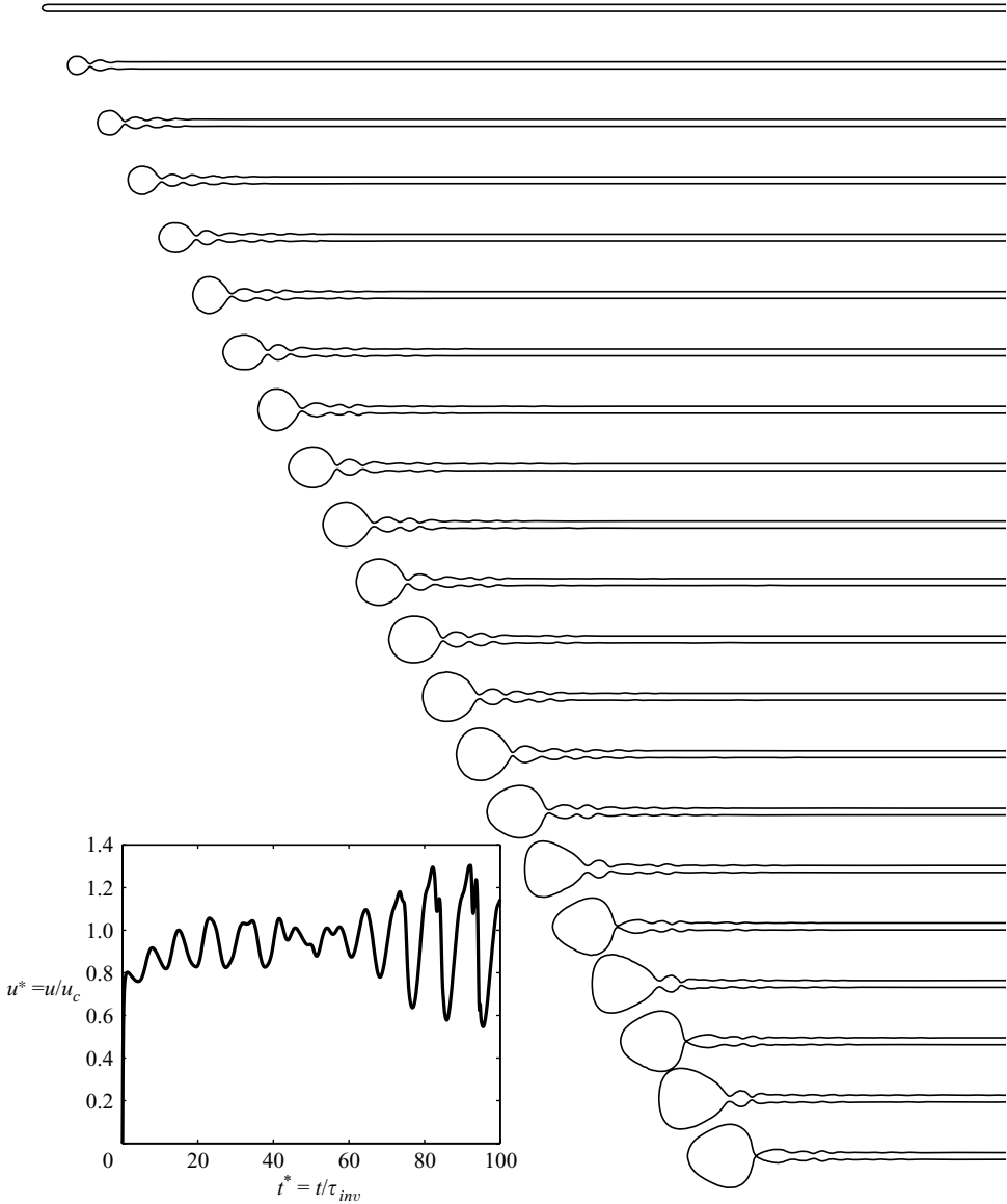
FIGURE 19. Sequence of the film profiles for Oh=0.01 in time increments of \delta t = 5t_{inv} ; (inset) tip speed versus time. The capillary waves are more pronounced and begin to interact with the rim after an initial transient. This interaction becomes more violent as time progresses and eventually causes breakup. (Inset) The evolution of the tip speed resulting from the rim–wave interaction.
