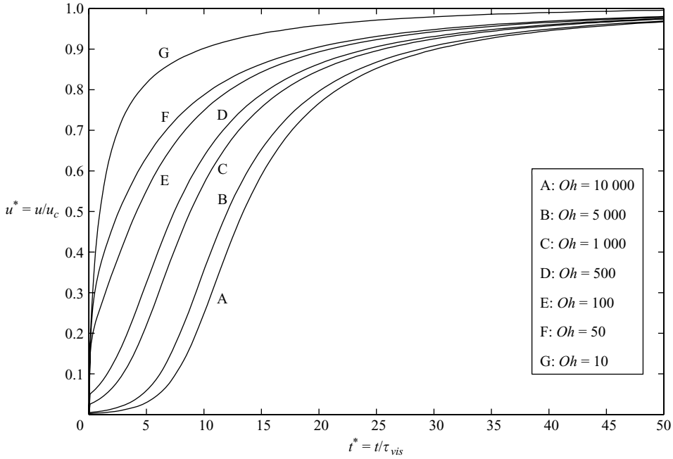
FIGURE 10. Speed at the film edge as a function of time for different values of Oh , with initial hole radius of R_0 = 50H . The higher the Oh the slower the approach towards the Taylor–Culick speed u_c .
