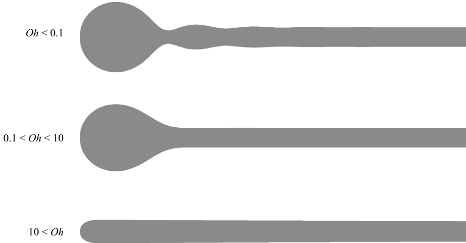
FIGURE 2. Schematic illustration of the three distinct regimes obtained for a retracting sheet by Brenner & Gueyffier (1999). As Oh progressively increases, the capillary waves and then the rim disappear through the action of viscosity.
