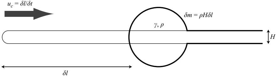
FIGURE 4. Retraction of a planar film. In time \delta t , the tip of the film moves by a distance \delta l = U_c \delta t . The mass of the fluid (per unit length) accumulated in the rim during that time is \delta m = \rho H \delta l .
