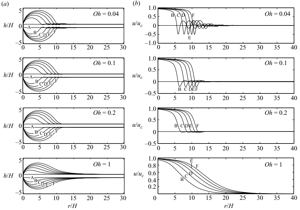
FIGURE 17. Evolution of the film boundaries and midplane velocities for moderate Oh in time increments of \delta t = 20 \tau_{mv} . Curves A to F correspond to times t^* = t/\tau_{mv} = 0, 20, 40, 60, 80 and 100 , respectively. The initial hole radius is R_0 = 50H . Note the generation of the capillary waves that are most pronounced for Oh = 0.04 and the associated oscillations in the midplane velocities. As Oh is increased, the capillary waves diminish and the rim begins to diffuse towards the bulk of the film.
