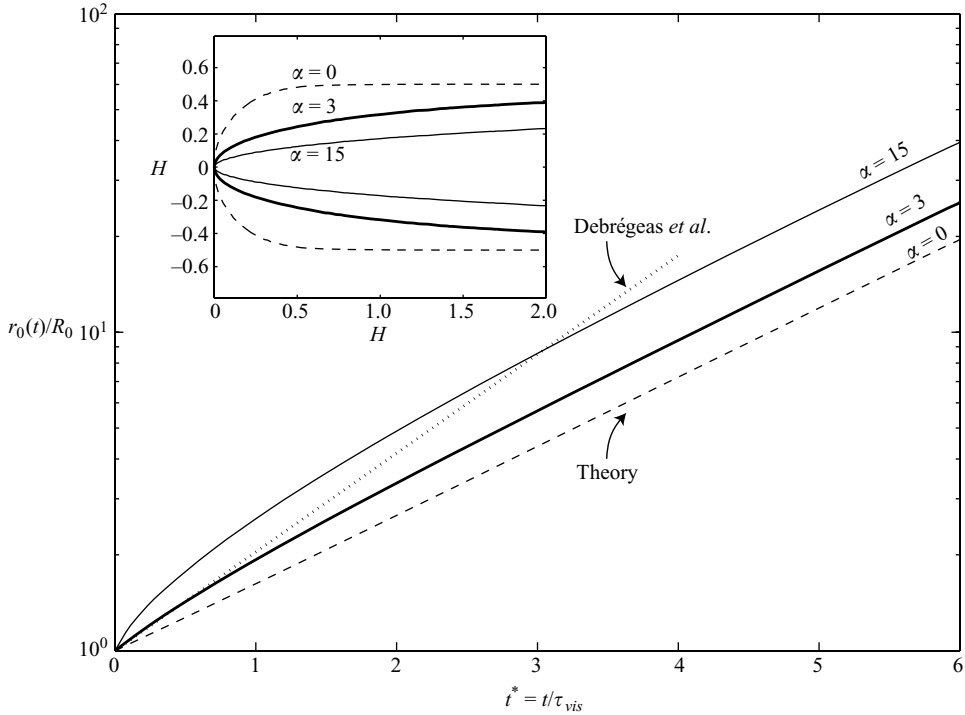
FIGURE 14. Effect of the initial film profile (as specified by \alpha ) on sheet retraction. Hole radius versus time for Oh = 8 \times 10^3 and R_0 = 40H . The inset shows the corresponding initial film profiles in the vicinity of the tip. A more pointed initial film profile retracts faster until its tip relaxes to a semi-circular cap; thereafter, the film retracts at the theoretically predicted rate shown by the dashed curve, corresponding to (3.30). The dotted line indicates the experimentally observed retraction rates reported by Debrégeas et al. (1995).
