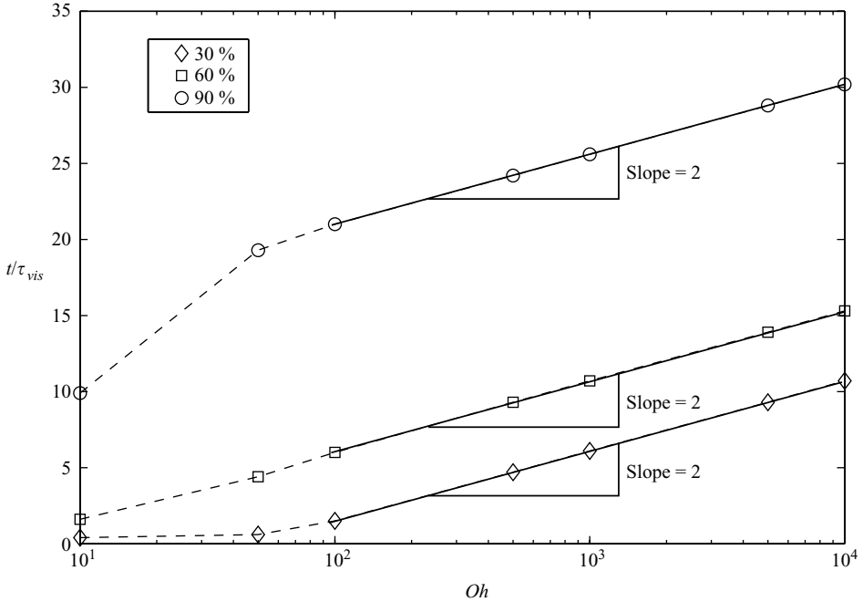
FIGURE 12. Time to reach 30 %, 60 % and 90 % of the Taylor–Culick speed versus Oh for simulations with R_0 = 50H . For Oh \geq 100 , there is logarithmic dependence on the Ohnesorge number, confirming the theoretically predicted retraction rate (1.3).
