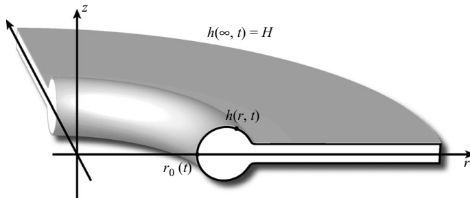
FIGURE 8. Circular sheet geometry. A circular hole expands on a flat fluid sheet owing to the radial surface tension force that acts on its toroidal edge.
