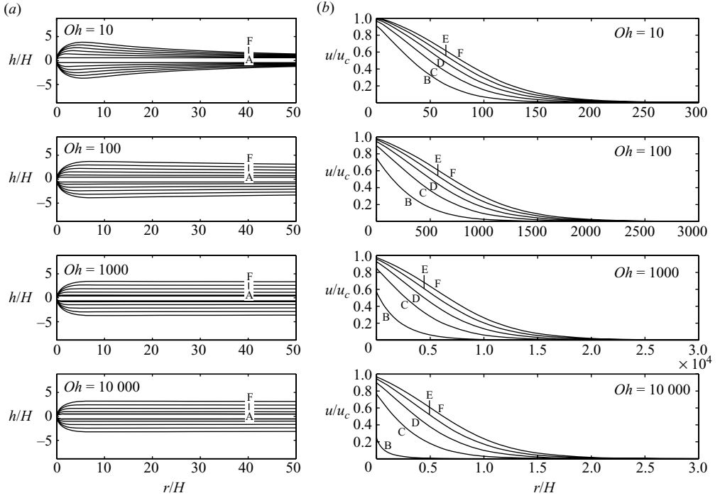
FIGURE 9. Evolution of the film boundaries (panel a ) and midplane speeds (panel b ) for high Oh and initial hole size R_0 = 50H in time increments of \delta t = 10 \tau_{vis} . Curves A to F correspond to times t^* = t/\tau_{vis} = 0, 10, 20, 30, 40 and 50 , respectively. Distances are scaled by the film thickness H . As Oh is progressively increased from 10 to 10^4 , the rim becomes less pronounced and diffuses towards the bulk. Concurrently, the region of influence of the disturbance caused by the tip motion extends further into the film and its lateral extent is proportional to Oh .
