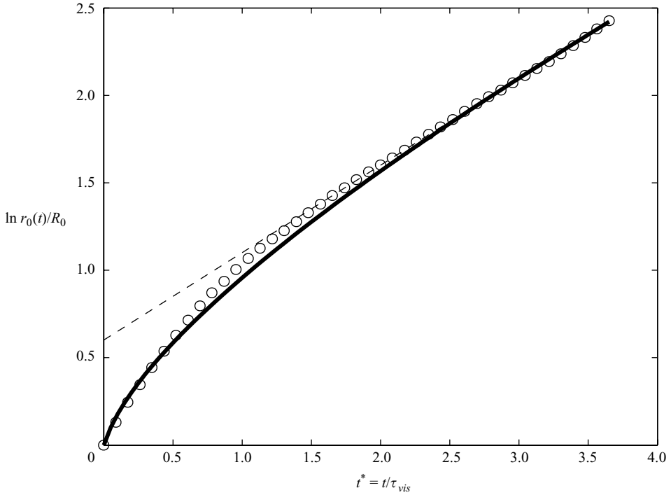
FIGURE 15. Hole radius versus time. The experimental data of Roth et al. (2005) is presented as circles, and our simulations for Oh = 1000 and \alpha = 32 by a solid line. After an initial transient of order \tau_{vis} = \mu H / 2\gamma , the retraction rate decreases to that predicted by (3.30), corresponding to the dashed line.
