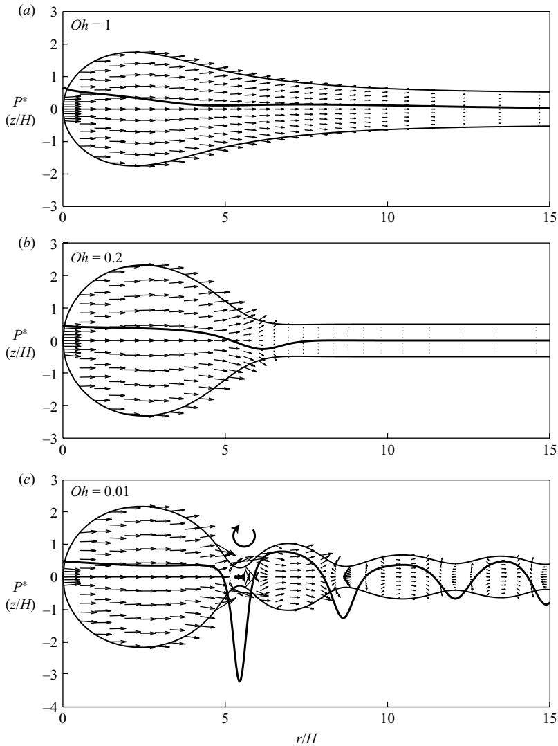
FIGURE 18. Velocity field and midplane pressure for (a) Oh = 1.0 , (b) Oh = 0.2 and (c) Oh = 0.01 . The velocity field is depicted by the arrows and the curve corresponds to the dimensionless pressure P^* = Hp/\gamma along the film midplane. For Oh = 1 (a), a monotonic decrease in the pressure prohibits the formation of a rim, which diffuses towards the bulk of the film. As Oh decreases, a rim begins to form due to the pressure drop at the rim neck (b). For Oh = 0.01 (c), vorticity generates capillary waves that are connected to the rim via a neck region. Note the pressure lows in the neck regions produced by the high local curvatures.
