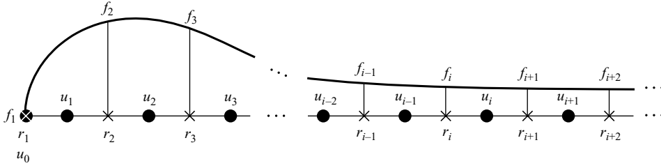
FIGURE 22. The staggered grid used for the computation. The values of f_i are prescribed at the mesh points r_i and the values of u_i are prescribed at (r_i + r_{i+1})/2 .
