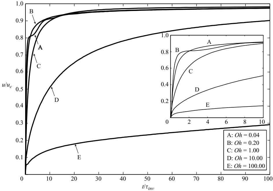
FIGURE 16. Speed of the film tip versus time since rupture for moderate Oh . Note the relatively slow retraction of the Oh = 100 film. (Inset) Early stages of retraction. When Oh = 0.04 , there is a brief reduction in the rate at which the film approaches u_c , due to the production of capillary waves ahead of the rim.
