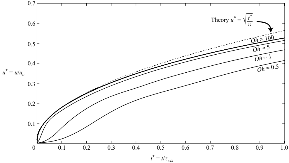
FIGURE 5. Plot of the tip velocity versus time during the early stages of retraction for different Ohnesorge numbers. The plots for Oh = 100, 500, 1000 and 10000 are indistinguishable. The dotted curve shows the theoretical result u^* = \sqrt{t^*/\pi} , which is in good agreement with numerics up to a time t \approx 0.4\tau_{vis} , where \tau_{vis} = \mu H/2\gamma .
