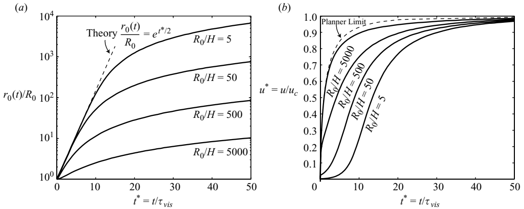
FIGURE 13. Variation of initial hole size for Oh = 1000 : (a) hole radius versus time and (b) tip speed versus time. For small initial hole radii, the agreement with the theoretically predicted exponential rate lasts for longer times. For larger initial radii, the retraction speed rapidly approaches the planar limit considered in §2.
