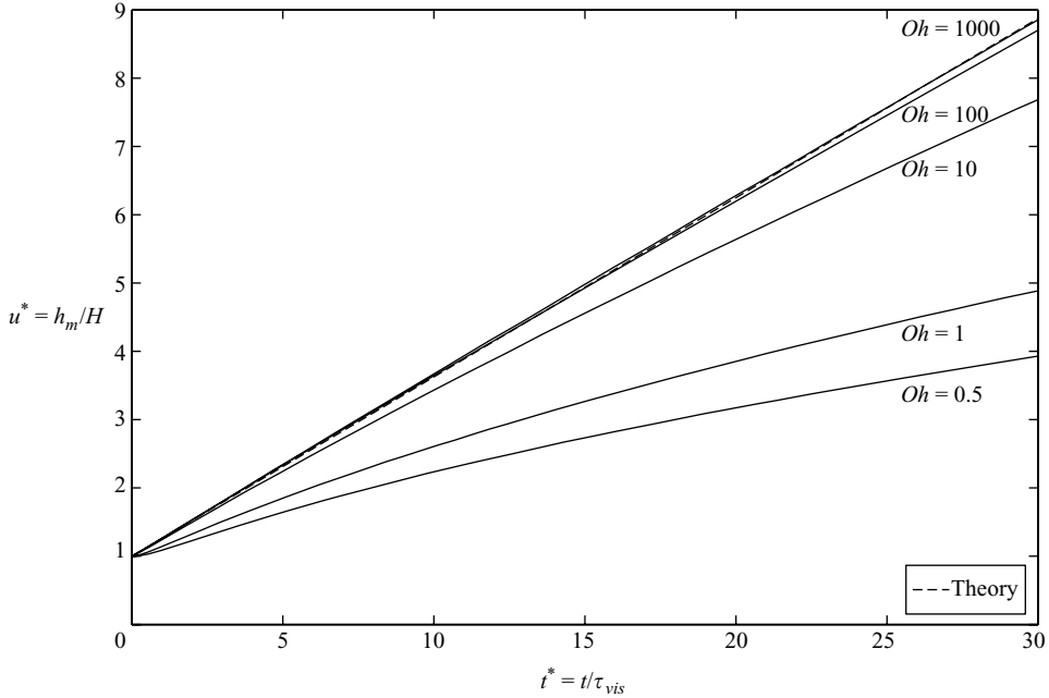
FIGURE 7. Maximum film thickness h_m versus time for different Ohnesorge numbers. In the high Oh limit, h_m grows linearly in time, confirming the theory represented by the dotted line that corresponds to (2.28). The numerical results (solid curves) at Oh = 0.5, 1.0, 10, 100 and 1000 correspond to profiles with \kappa_0 = 2.1 .
