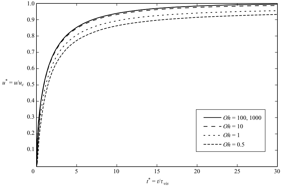
FIGURE 6. Velocity of the film edge for different Ohnesorge numbers. In the high Oh limit the velocity curves become indistinguishable.
