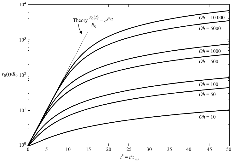
FIGURE 11. Hole growth versus time for different Oh , for an initial hole size R_0 = 50H . The higher the Oh , the longer the hole grows according to the exponential law (1.3) as deduced by Debrégeas et al. (1995).
