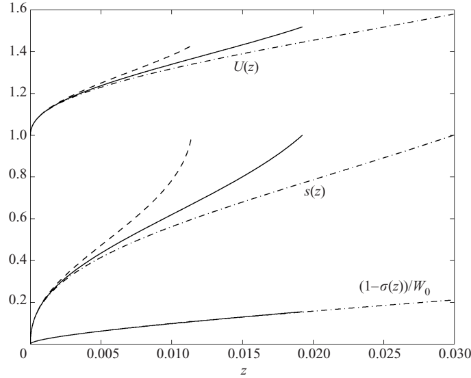
FIGURE 7. Theoretically predicted z -dependence of the scaled surface tension deficit (1-\sigma(z))/W_0 = (\sigma_0 - \sigma')/(\Delta\sigma W_d) , boundary layer thickness s(z) and inviscid core velocity U(z) for Stokes numbers \mathcal{L} = \nu V/(ga^2) = 0.04 (dashed line), 0.062 (solid line) and 0.1 (dash-dot line) that span the experimental parameter regime.
