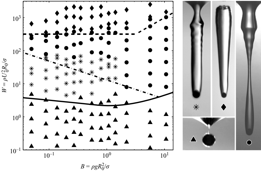
FIGURE 8. Regime diagram indicating the dependence of the observed cavity type on B and W for \theta_a = 120^\circ . The triangle, asterisk, circle and diamond symbols denote the quasi-static, shallow seal, deep seal and surface seal regimes, respectively. The dash-dotted line is defined by (6.23a), and the solid curve by equating the pinch-off times defined by (5.5) and (6.3) for \alpha = 0.065 ( \theta_c = 166^\circ ), \theta_a = 120^\circ and C_a = 1/2 . The dashed line is given by the empirical fit W = 320 at low B (present study) and F = (1/6400)\tilde{D}^{-2} at high B (Birkhoff & Isaacs 1951).
