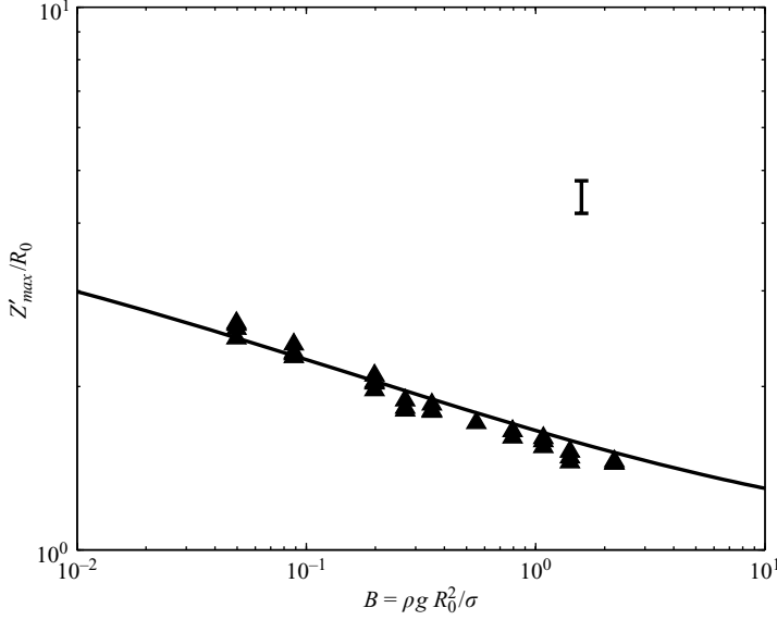
FIGURE 12. Penetration depth of a low speed ( W \ll 1 ) impactor with a quasi-static cavity. The triangles denote the experimental data for impacting spheres ( 10^{-4} < W < 10^{-2} ), and the solid curve is defined by (5.3) for \theta_a = 120^\circ , corresponding to the measured advancing contact angle. A characteristic error bar is shown.
