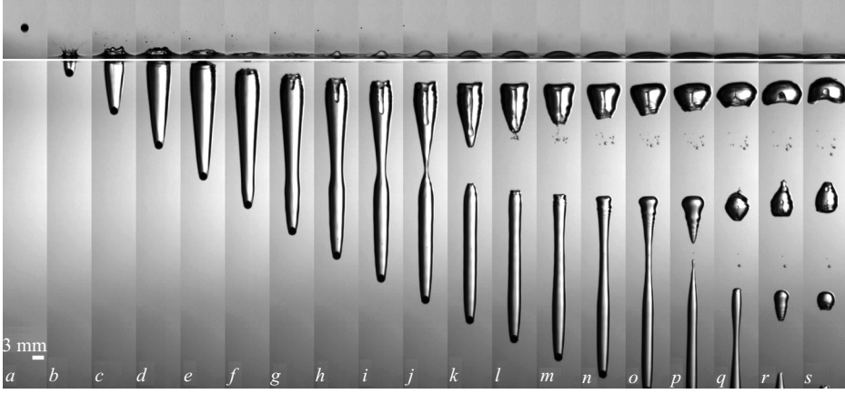
FIGURE 7. Surface seal impact cavity. Video sequence of the water entry of a hydrophobic steel sphere at low B ( R_0 = 0.10 cm, \rho_s = 7.7 g cm ^{-3} , U_0 = 540 cm s ^{-1} ). The time between successive images is 1.9 ms; W = 420 ; B = 0.14 .
