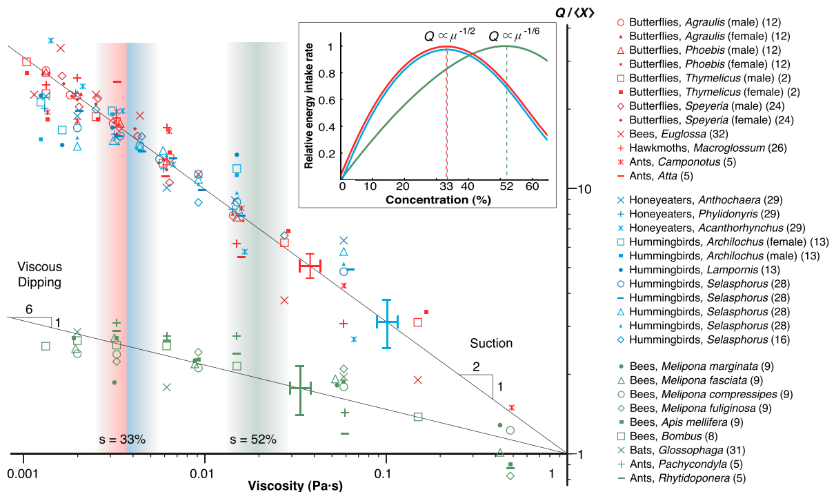
Fig. 2. The dependence of scaled volumetric flow rate Q/\langle X \rangle on nectar viscosity \mu (2, 5, 8, 9, 12, 13, 16, 24, 26, 28, 29, 31, 32). The red points represent data for active suction, the blue points for capillary suction, and the green points for viscous dipping. The slopes of the expected lines for suction and viscous dipping are -1/2 and -1/6 , respectively. Inset: Optimal concentrations for suction feeding (33%) and viscous dipping (52%), calculated from the dependence of relative energy intake rate on nectar viscosity, are denoted by vertical bands. Characteristic error bars are shown.
