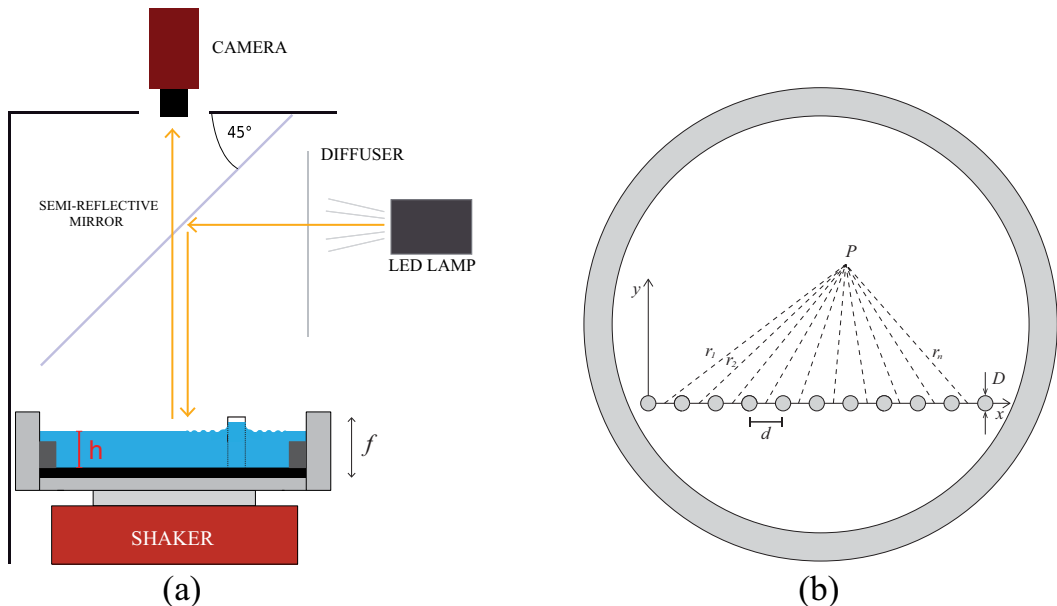
FIG. 1. (a) Experimental arrangement [27]. The fluid bath is shaken using an electromagnetic shaker and imaged using a CCD camera through a 45^\circ semireflective mirror with diffuse illumination [12]. (b) Top view of the fluid bath shows the row of N protruding pillars of diameter D and center-to-center separation d .
